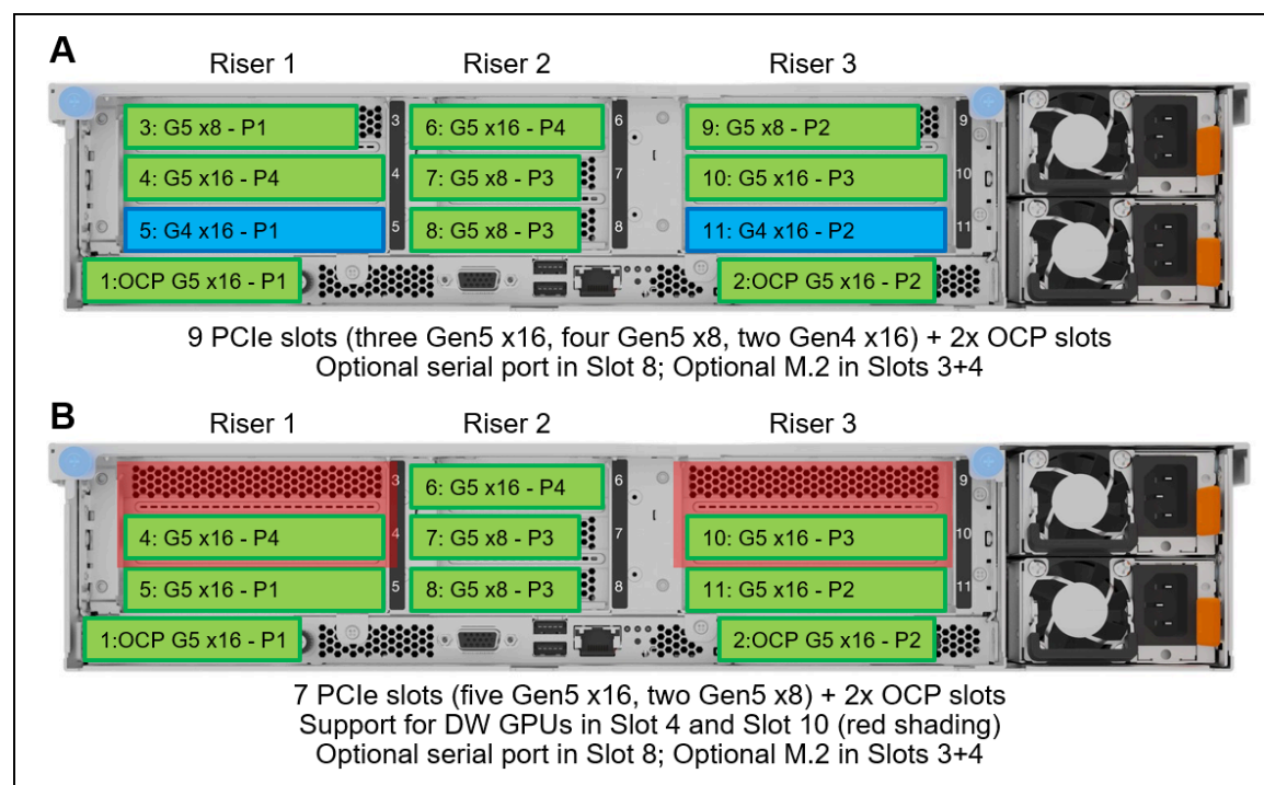
Figure 19. SR850 V4 with 6x Full Height slots + 3x Low Profile slots
