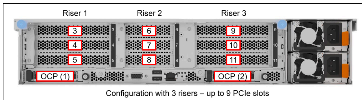
Figure 16. Slots in the SR850 V4
