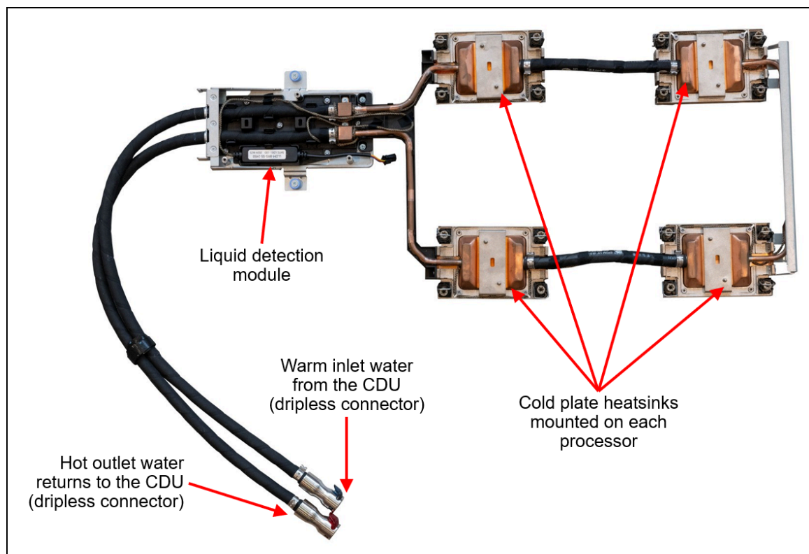
Figure 11. Lenovo Processor Neptune Core Module
