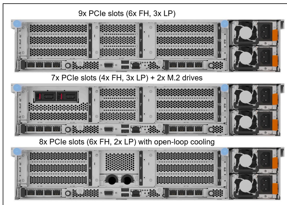
Figure 5. Rear configurations of the SR850 V4 - 3 risers
