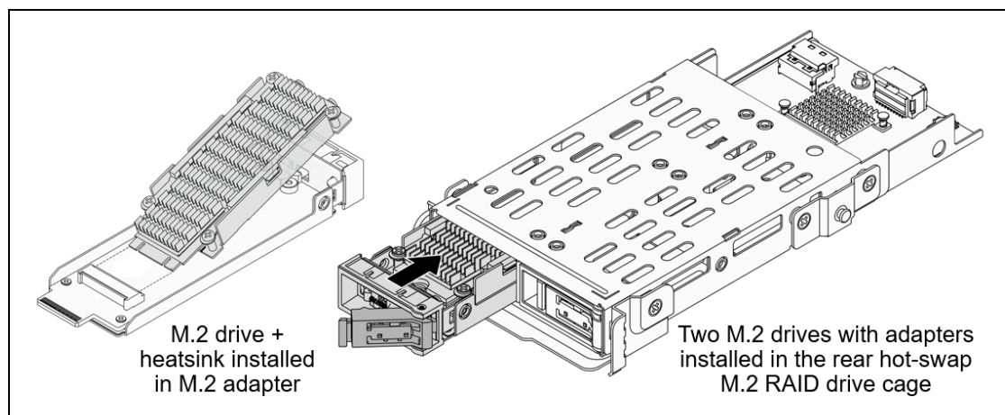
Figure 14. Rear hot-swap M.2 drive bays
