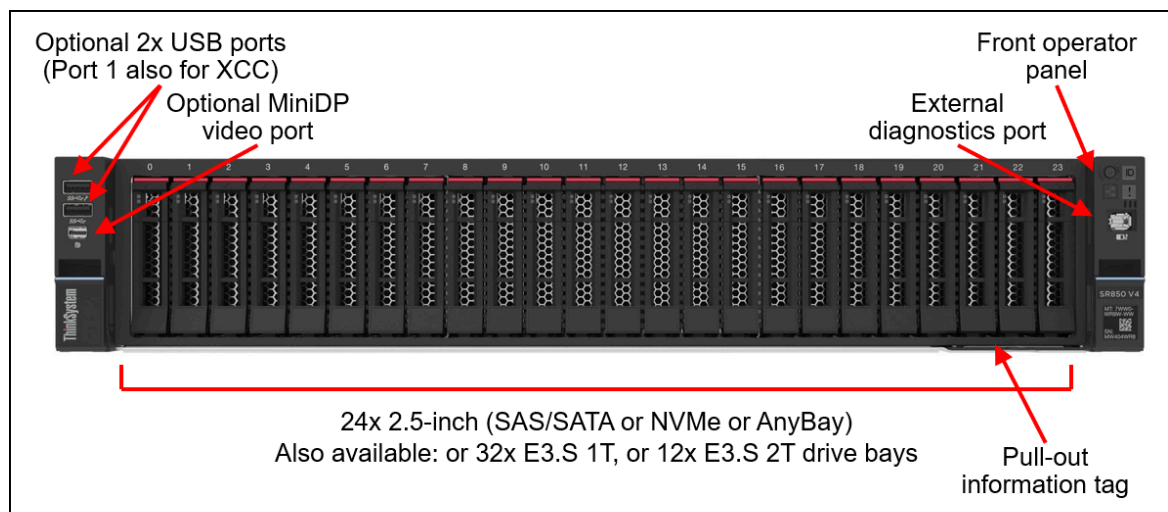
Figure 2. Front view of the ThinkSystem SR850 V4 with 2.5-inch drive bays
