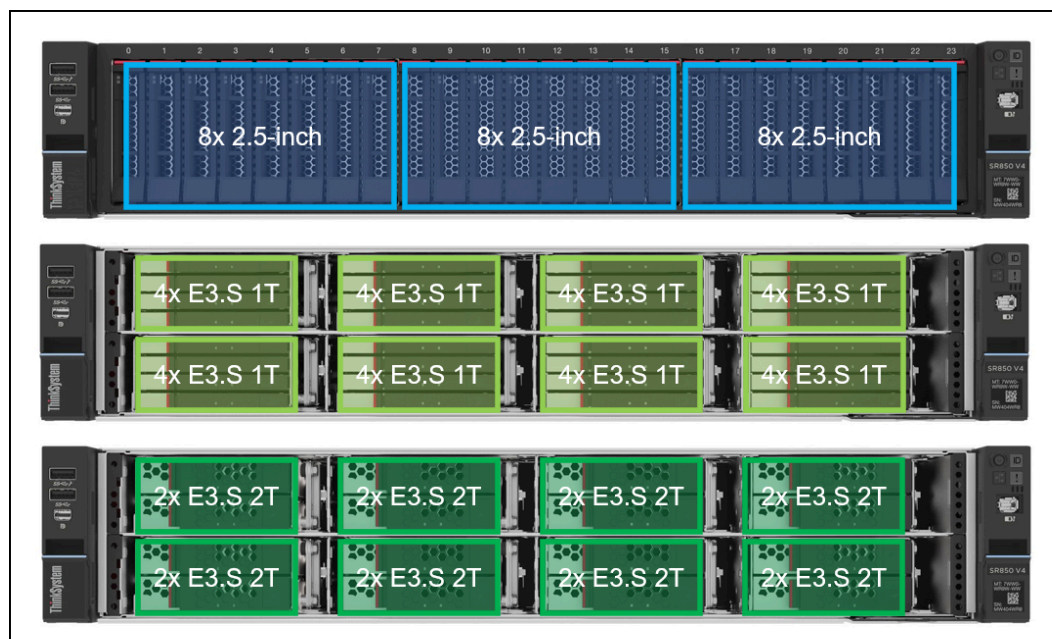
Figure 12. SR850 V4 drive bays
