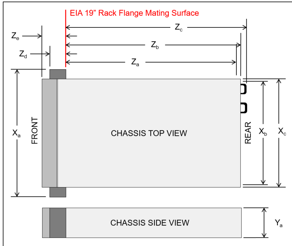
Figure 28. Server dimensions
