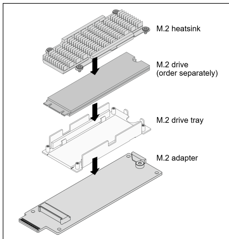
Figure 15. Components of the ThinkSystem V4 Hot Swap M.2 SATA/NVMe Drive Assembly Kit (4XH7A96837)
