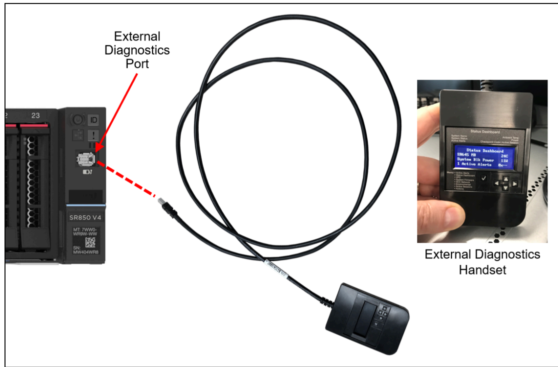
Figure 26. External Diagnostics Handset
