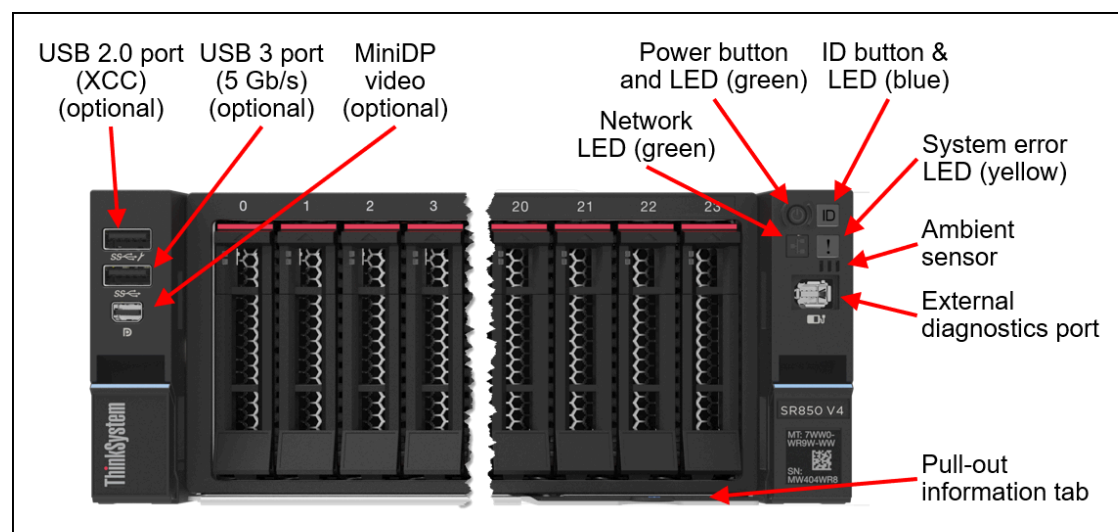
Figure 25. Front operator controls are on the left and right side of the server
