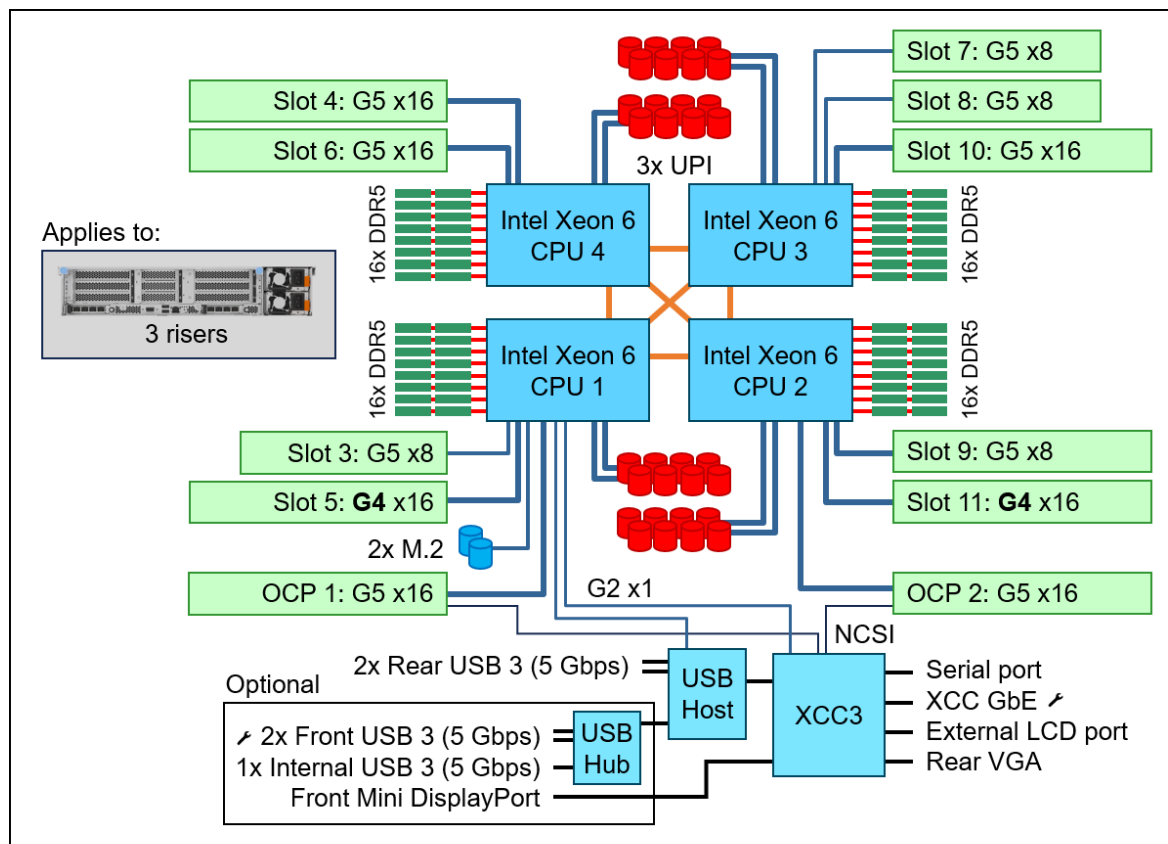
Figure 10. SR850 V4 system architectural block diagram - 3-riser configuration
