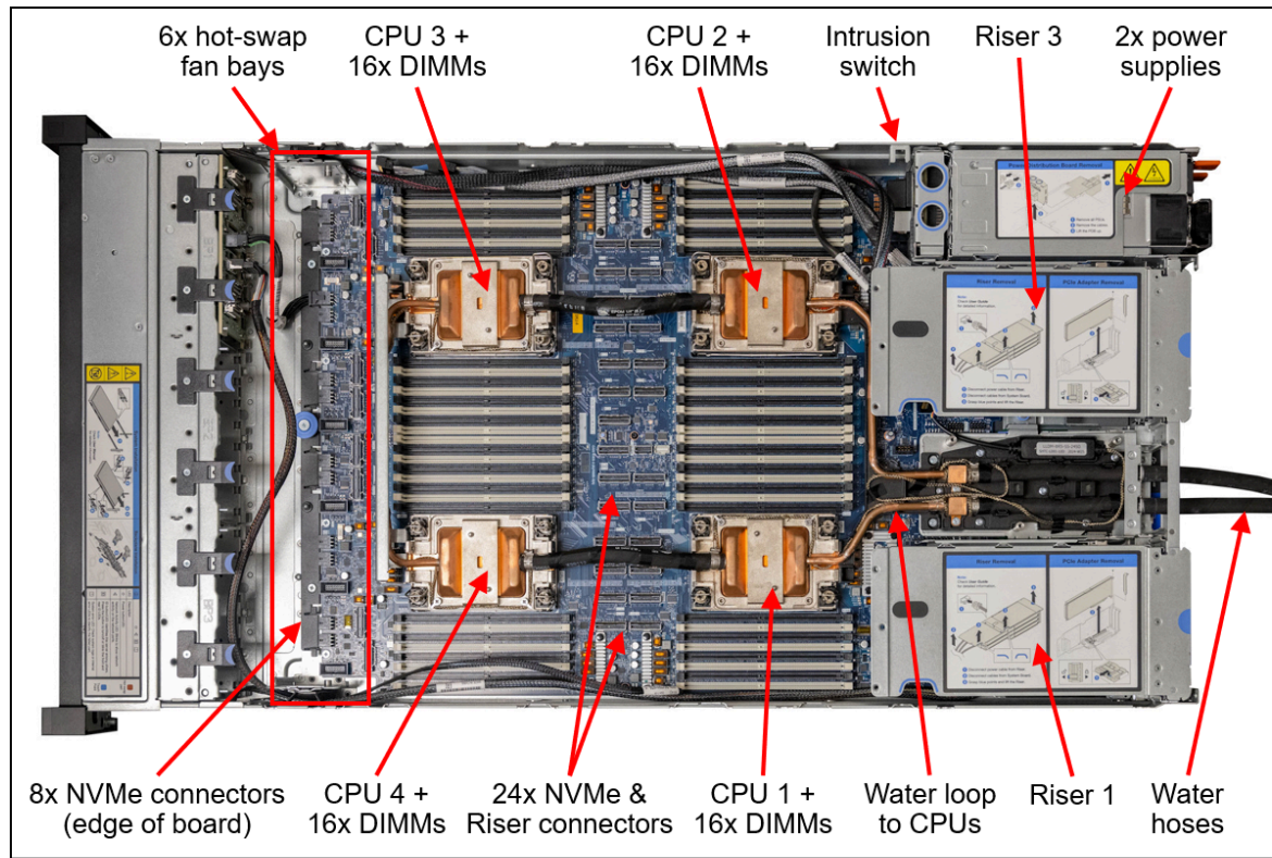
Figure 7. Internal view of the ThinkSystem SR850 V4 (shown configured with Lenovo Neptune Core open-loop water cooling)
