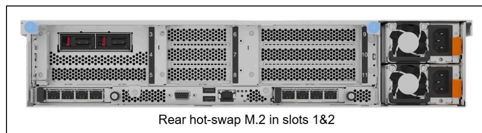
Figure 13. Hot-swap M.2 drive bays
